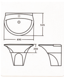
NEW [Water Basin] ▶ C L-771P (L610 (7Liter))
