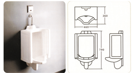
NEW [Urinal] ▶ C U-301 (8U410)
