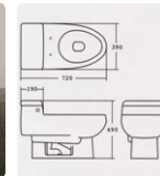
[Water Closet] ▶ CC-207 (C1210C) (6Liter)
