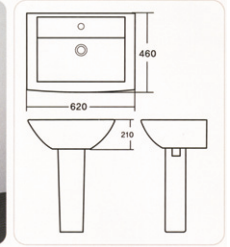
NEW [Water Basin] ▶ C L-902 (7Liter)
