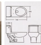
[Water Closet] ▶ CC-251 (C1210C) (6Liter)
