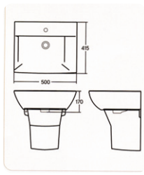
NEW [Water Basin] ▶ C L-336R P (6.5Liter)
