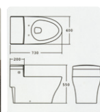
[Water Closet] ▶ CC-213 (6Liter)
