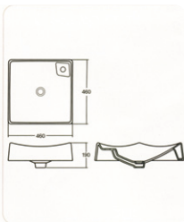
NEW [Water Basin] ▶ C L-851 (수평수전) (6Liter)
