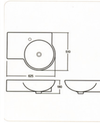
NEW [Water Basin] ▶ C L-450R (4.5Liter)
